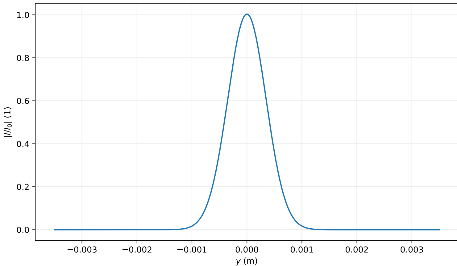
Intensity profile I(x=0, y, z=0.080)/I_0 , \text{Pin}=0.8\text{Pcr} , artificial time
